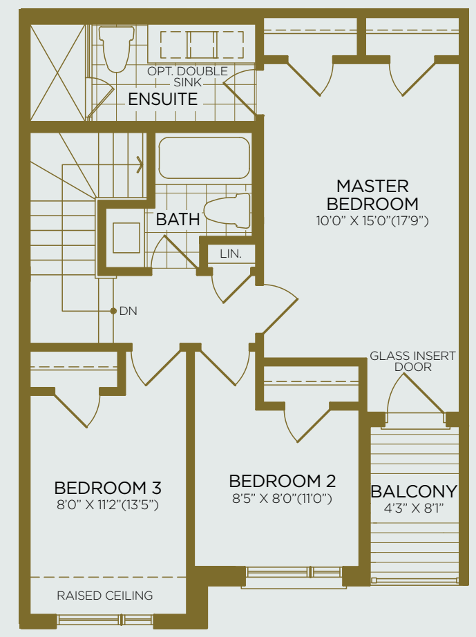
Upper Floor Elev. A
