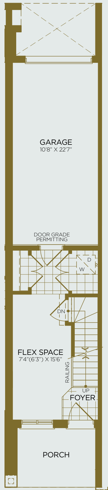
Entry Level Elev. A/B
