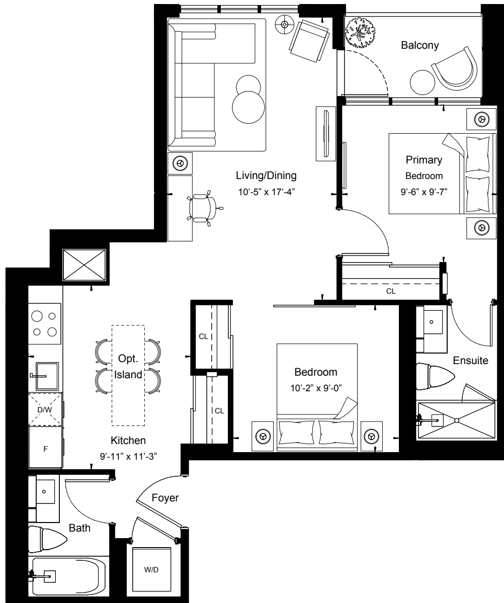
FLOORS 3-5
