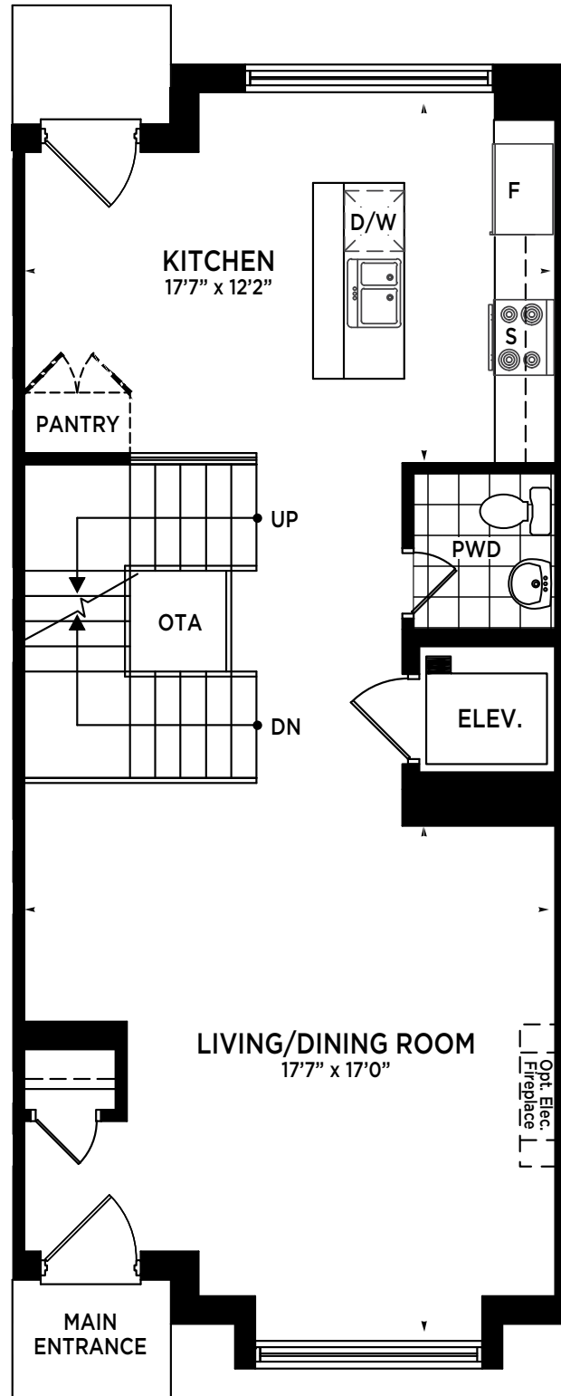
MAIN LEVEL
