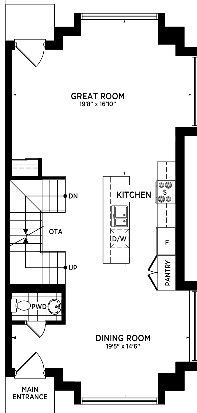
MAIN LEVEL
